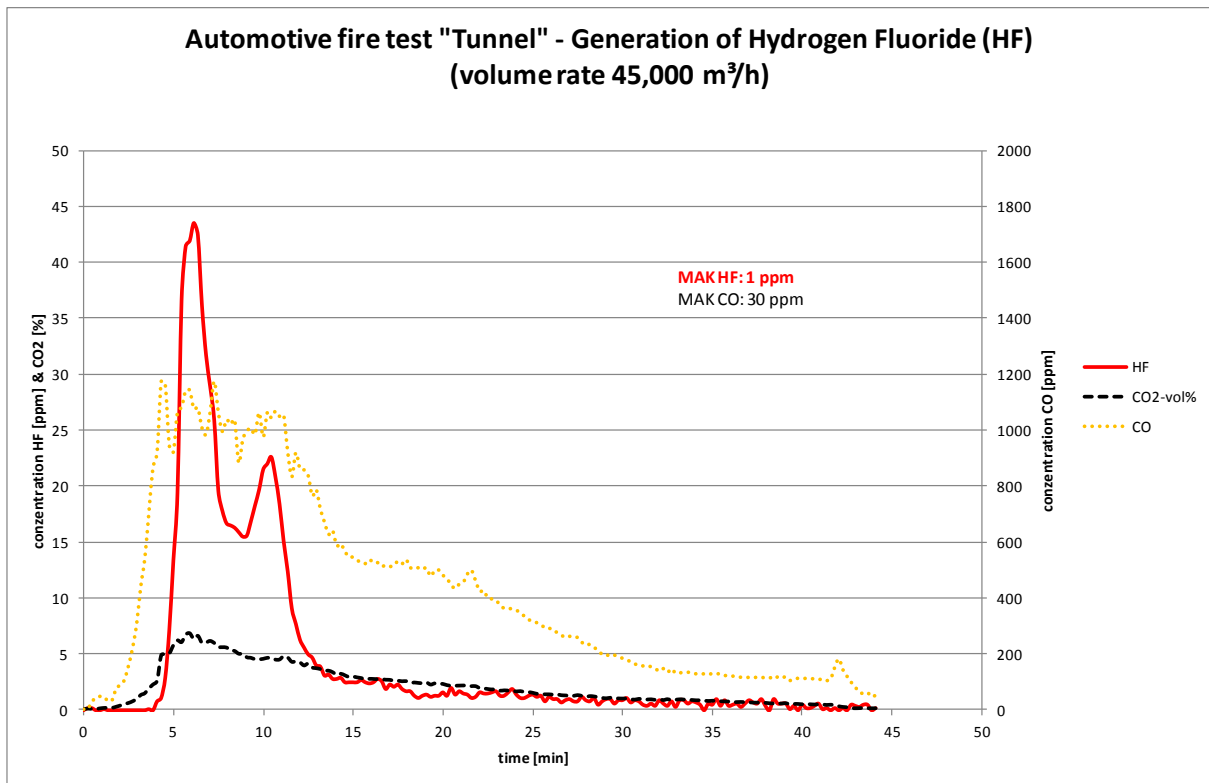
Fig. 1) Change over time of the combustion gases carbon monoxide (CO), carbon dioxide (CO 2 ) and hydrogen fluoride (HF)
